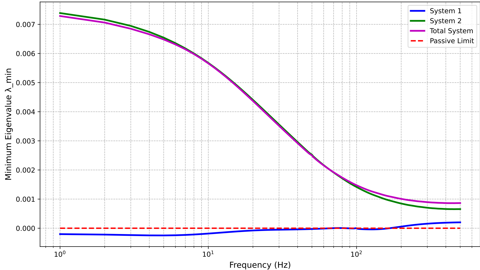
Passivity Evaluation via Minimum Eigenvalues
